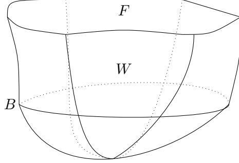
FIGURE 1. Domain W with boundary \partial W = F \cup B .
